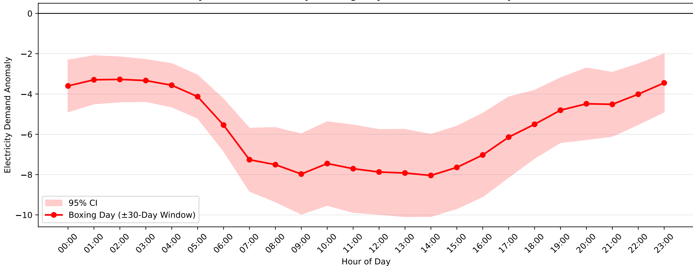
Botany Demand Anomaly: Boxing Day (2004-2017, \pm 30 -Day Window)
